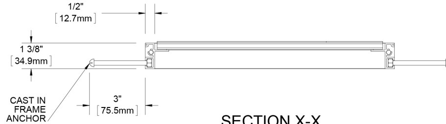
SECTION X-X
