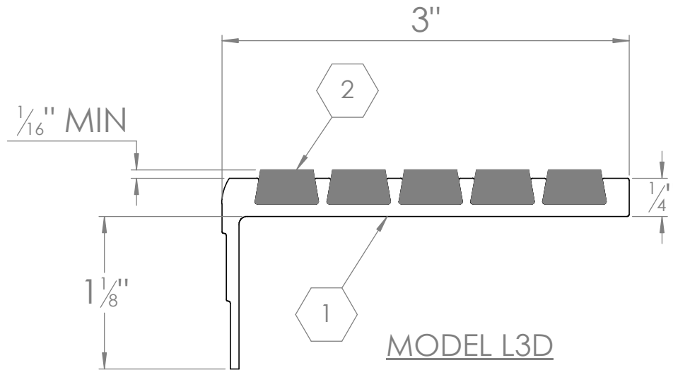
(SINGLE STAGE RIBBED ABRASIVE BARS)
